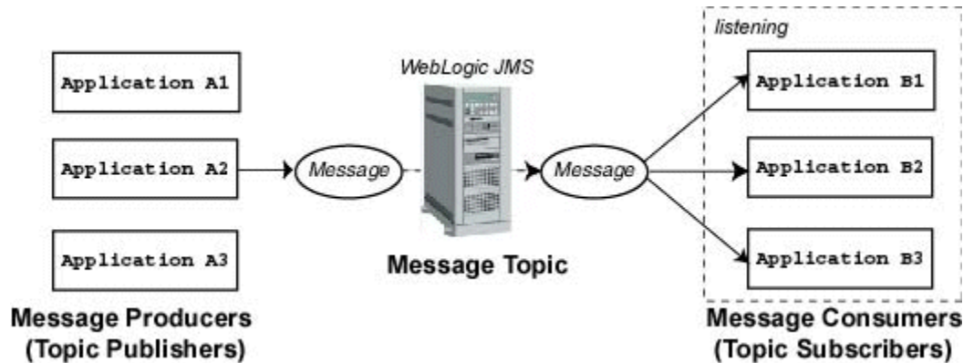
Figure 2-4 Publish/Subscribe (Pub/Sub) Messaging
