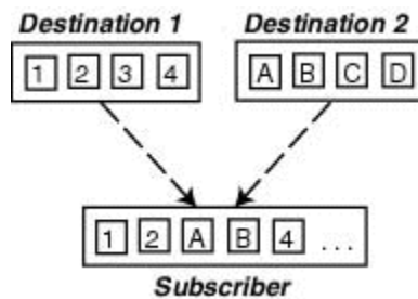
Figure 9-2 Multicasting Sequence Gap
