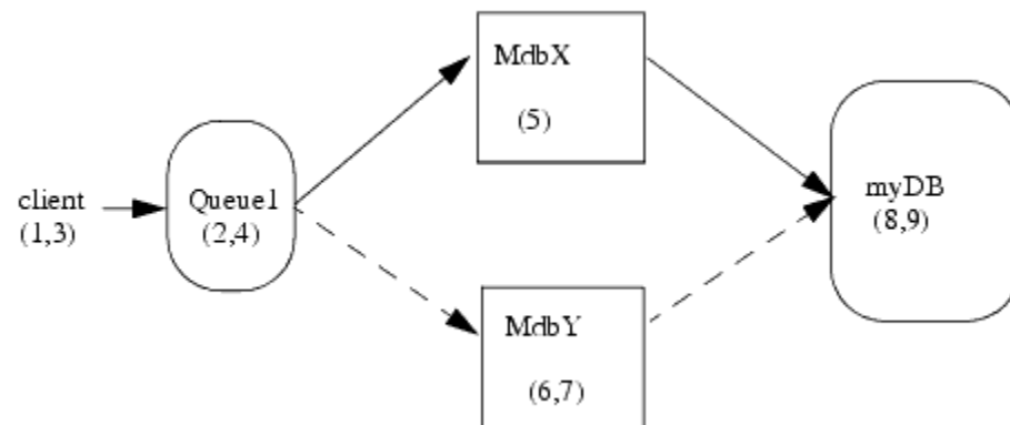
Figure 11-2 Workflow for Joe's Order Using Unit-of-Order
