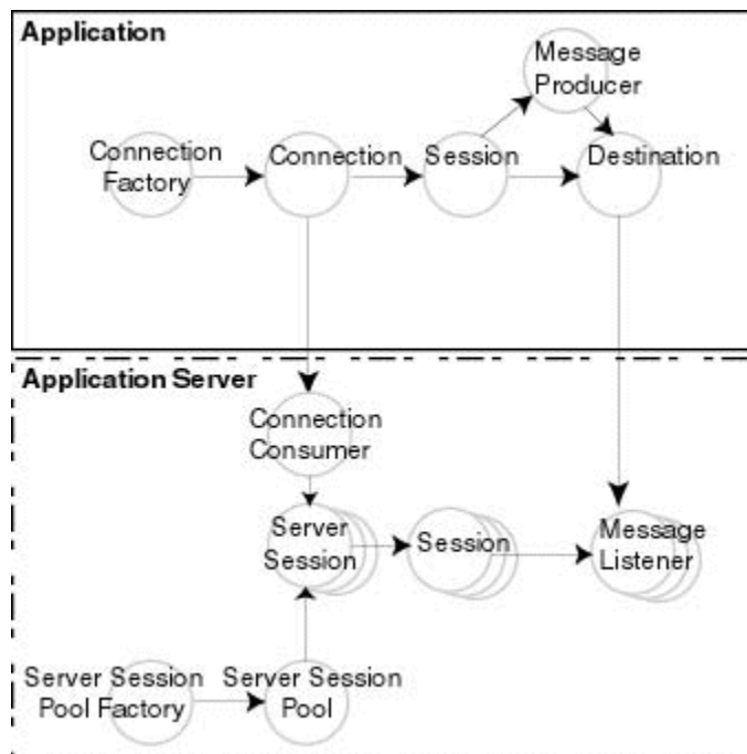
Figure A-1 Server Session Pool Facility
